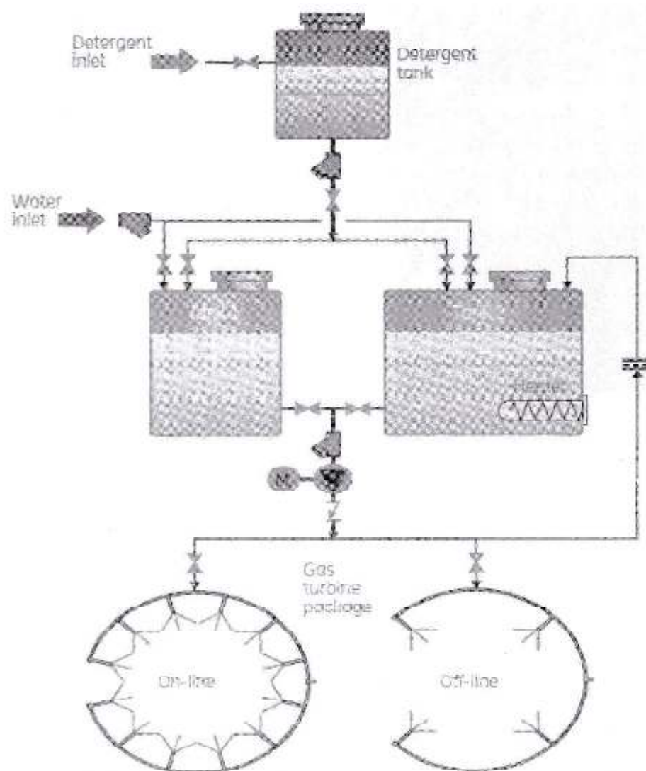
Fig.3 :Pictorial Representation of water wash system[14]
