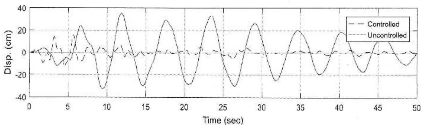
a) Top floor Displacement under the El-Centro Earthquake
