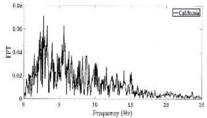
(b) Time history and FFT of California Earthquake
