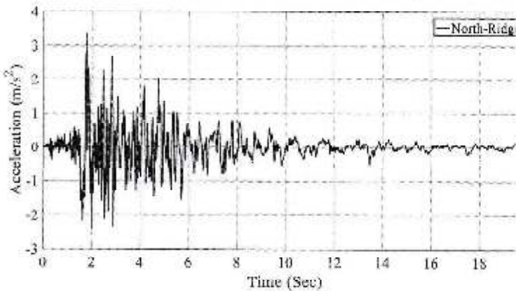
(c) Time history and FFT of North Ridge Earthquake
