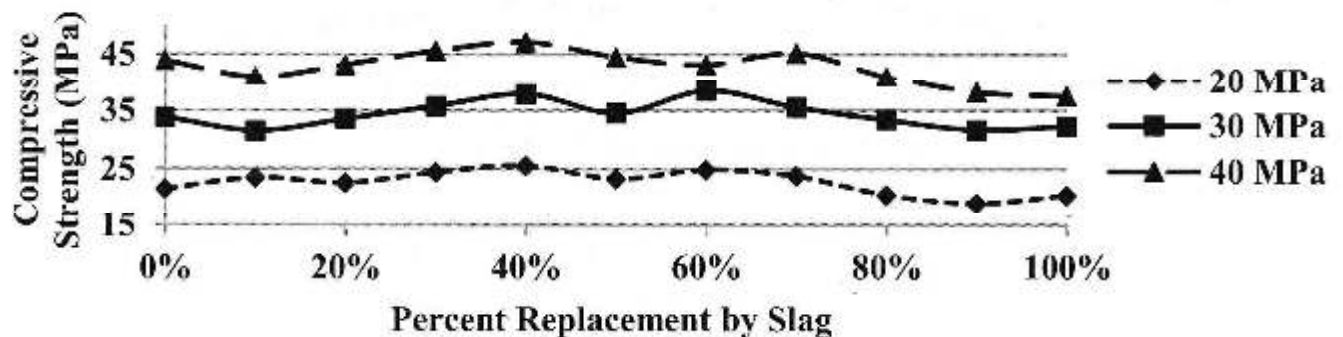
Fig. 3. Compressive strength variation vs. percent replacement by slag of coarse aggregate for curing age of 28 days
