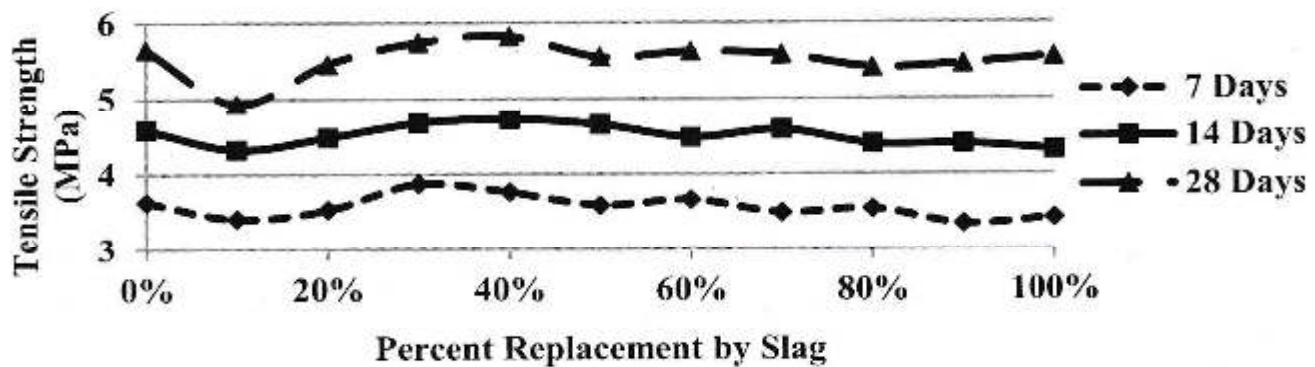
Fig. 5. Tensile strength variation vs. percent replacement by slag for 30MPa
