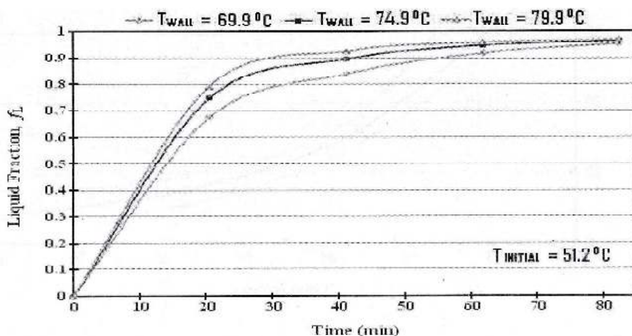
Fig. 6. Changes of the cumulative total liquid fractions with melting time for cases (1-3) in the long-finned LHTES unit.
