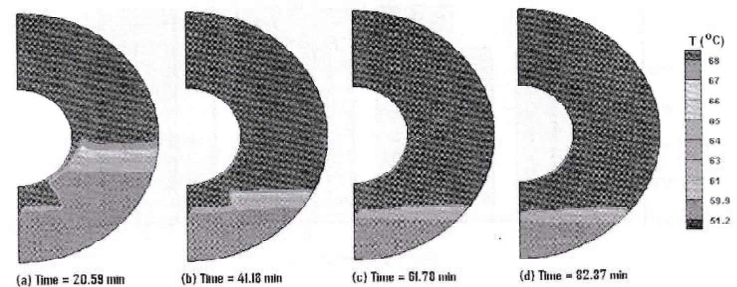
Fig. 8. 2-D views of the changes of the isotherms with time during the melting in a short-finned annulus for case4.
