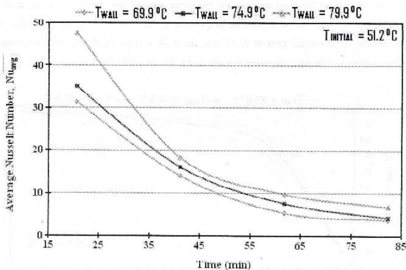
Fig. 5. Changes of the surface-averaged Nusselt numbers on the inner circular cylinder with melting time for cases (1-3) in the long-finned LHTES unit.
