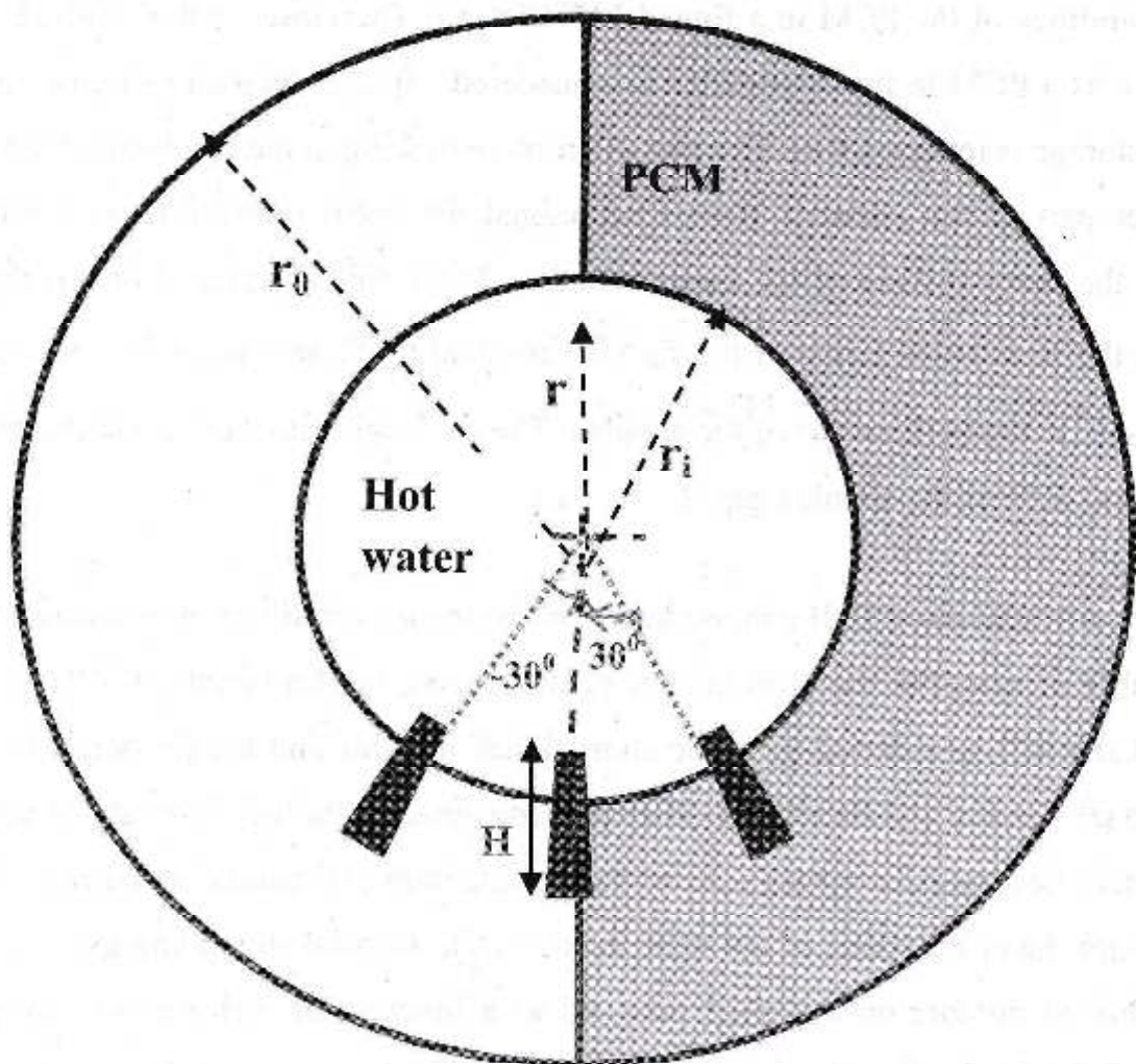
Fig. 1. Schematic view of the cross-section of the finned annulus where the blue part representing the computational domain.
