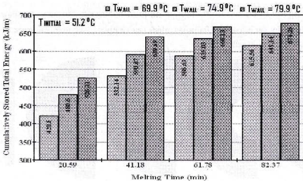
Fig. 7. Changes of the cumulatively stored total energies with melting time for cases (1-3) in the long-finned LHTES unit.
