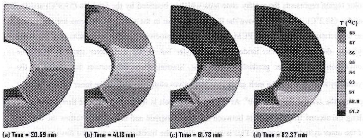
Fig. 2. 2-D views of the changes of the isotherms with time during the melting in a long-finned annulus for case1.
