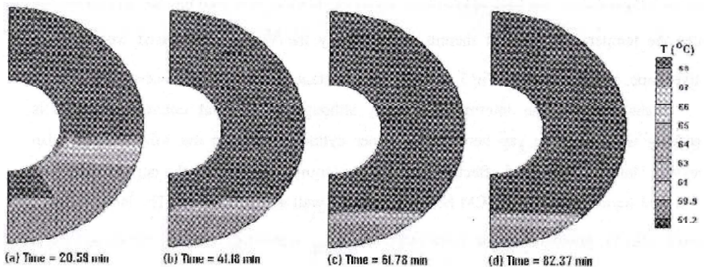
Fig. 4. 2-D views of the changes of the isotherms with time during melting in a long-finned annulus for case-3.
