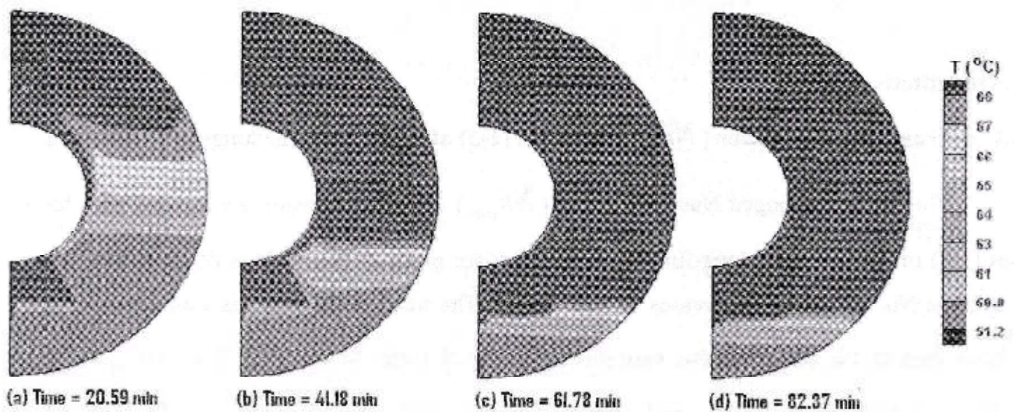
Fig. 3. 2-D views of the changes of the isotherms with time during melting in a long-finned annulus for case-2.
