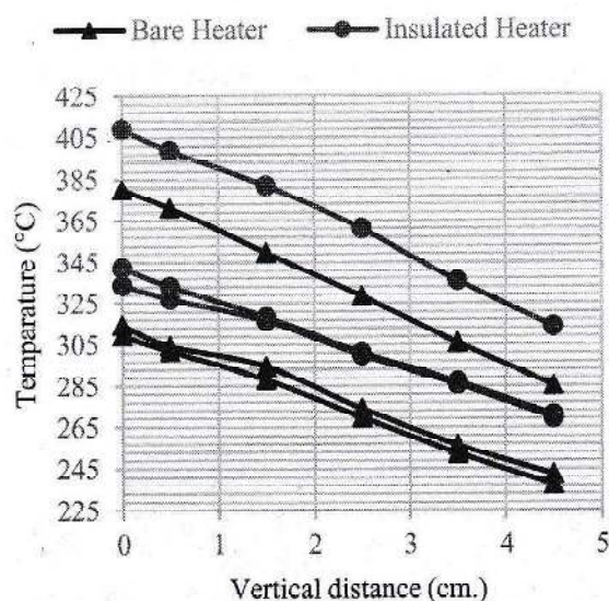
Fig. 8. Temperature Profile along Vertical Height for both Bare and Insulated Heater.
