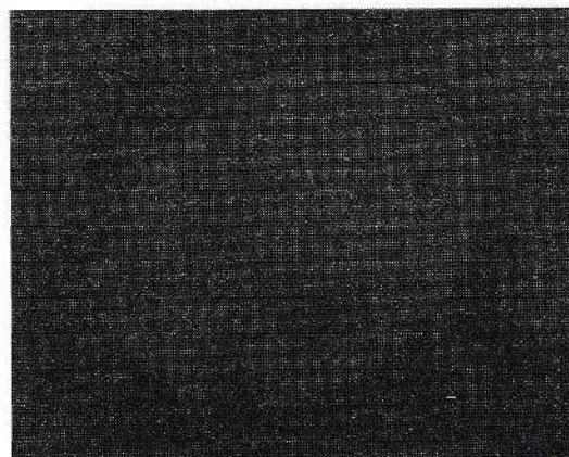
Fig. 18. 1 st iteration (when z = 0 )
