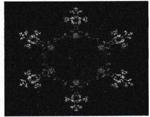
Fig. 11. Fractal crown
